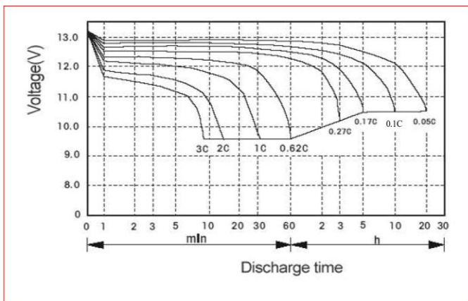
Discharge performance
