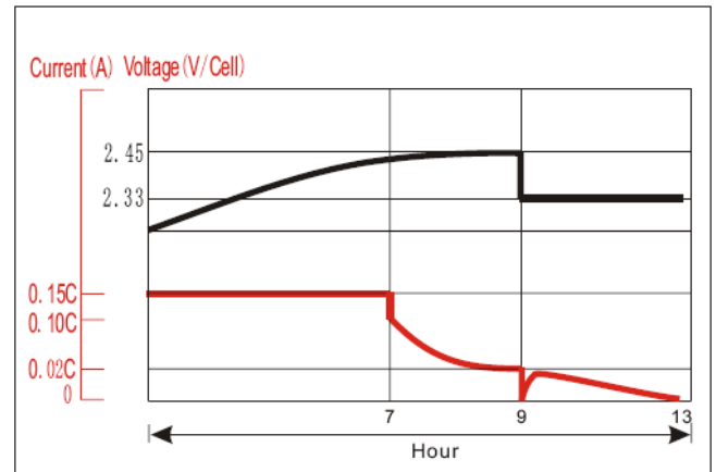
Charge performance
