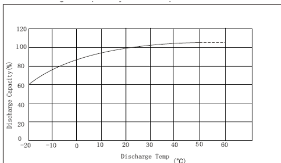
Discharge capacity Vs temperature
