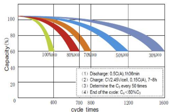
Cycle life Vs discharge depth
