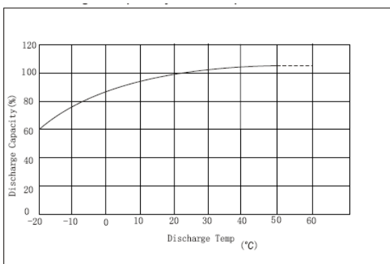
Discharge capacity Vs temperature
