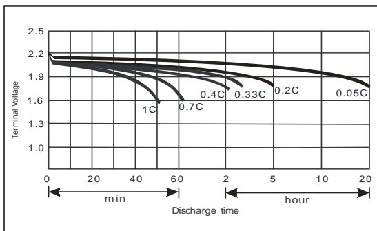
Discharge performance
