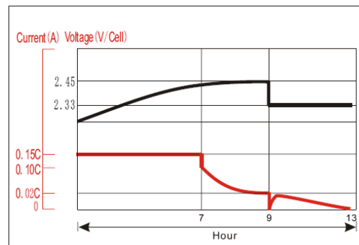
Charge performance
