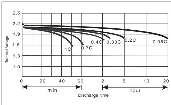
Discharge performance
