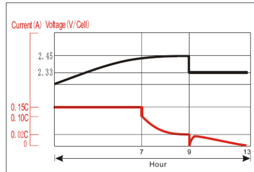
Charge performance
